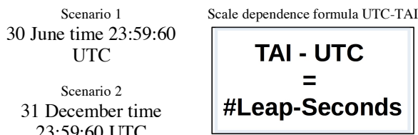
Figure 27 Scenarios of changes of the leap second and TAI-UTC dependence
