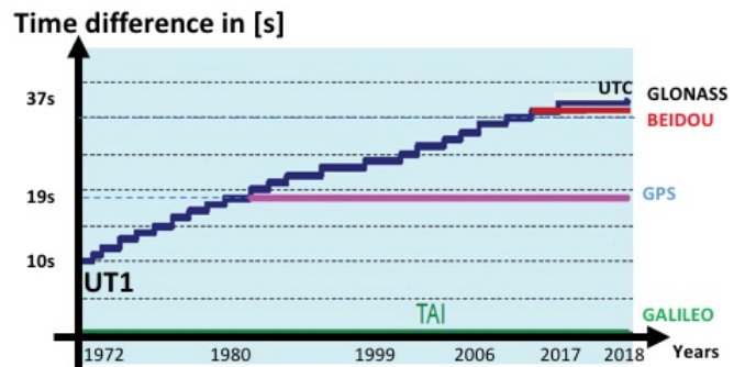
Figure 25 Historical evolution of the time scales
